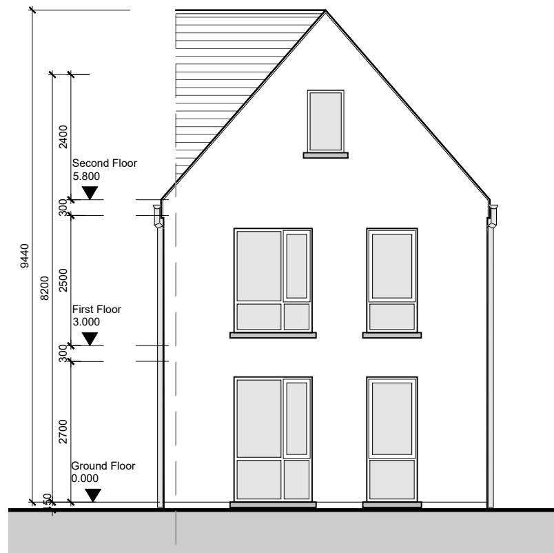
Front Elevation
