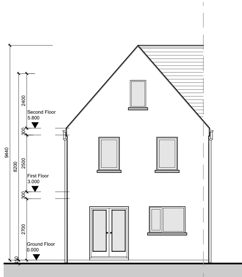
Rear Elevation
