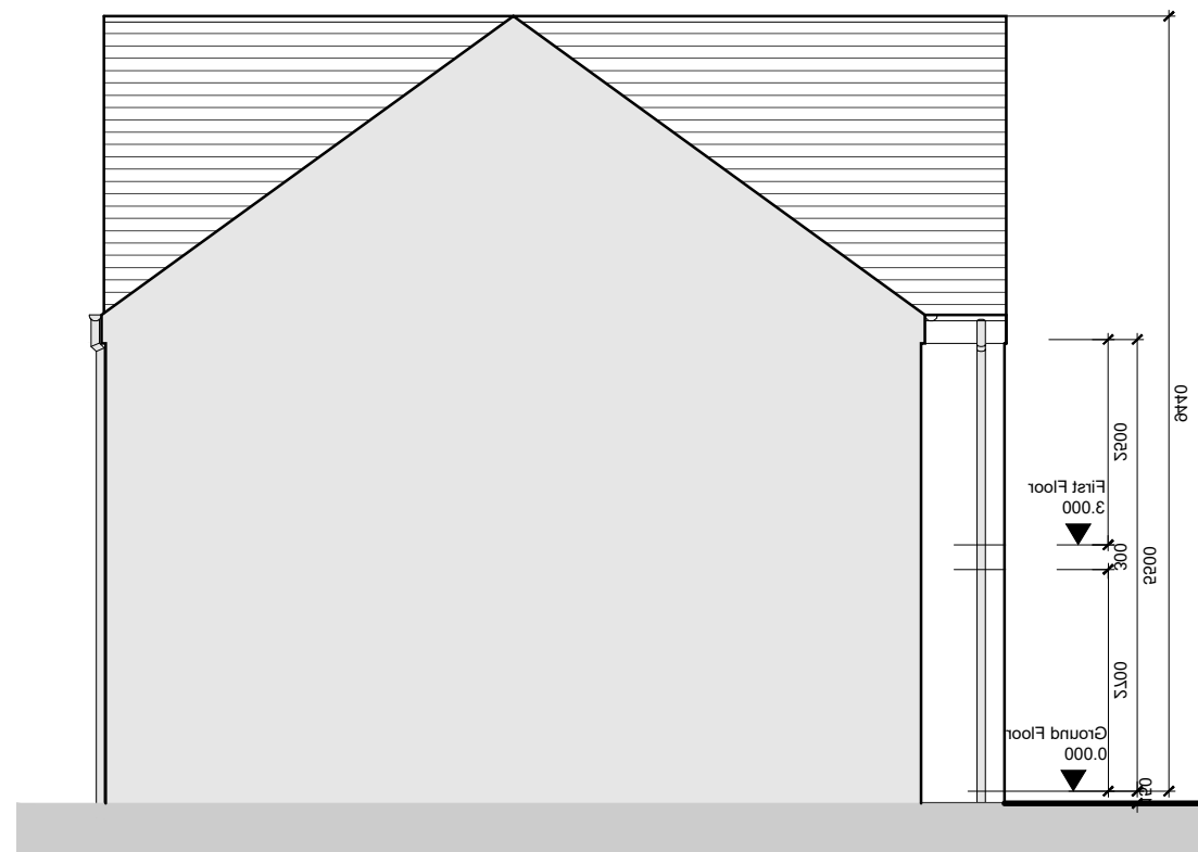
Side Elevation 02
